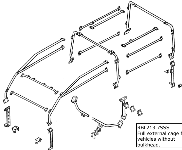
RBL108 7SSN Full external cage for vehicles with bulkhead
